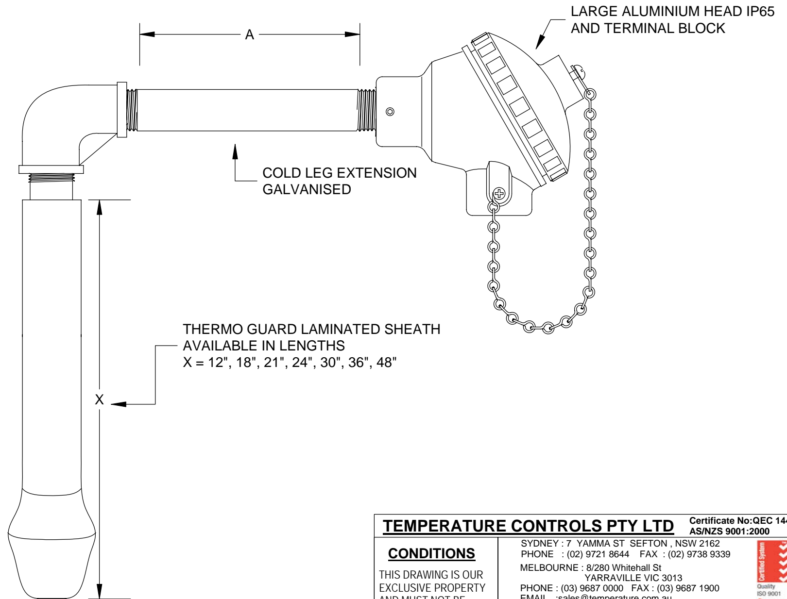
3mm DIA TYPE K THERMOCOUPLE LAMINATED AND REFRACTORY SHEATH FOR USE IN DIECASTING
